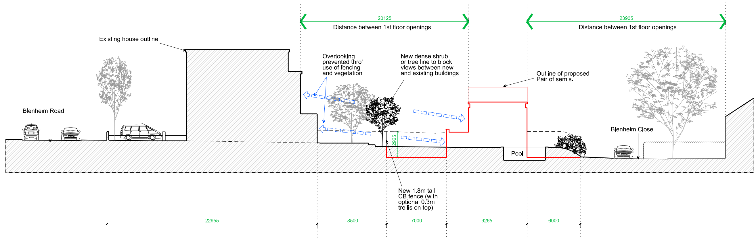
01 CROSS SECTION THROUGH THE SITE SCALE 1:250
